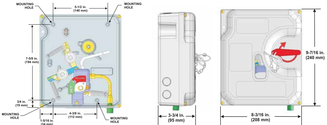
Figure 9. XV Control System Dimensions
