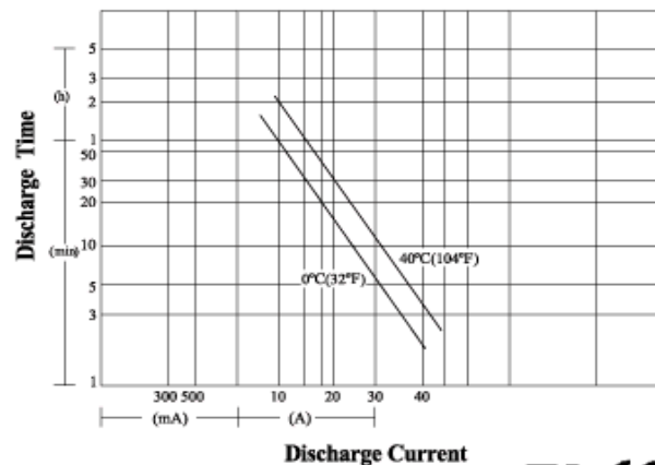
Discharge Characteristics (0°C/32°F, 40°C/104°F)
