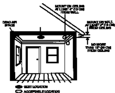
Figure 4: RECOMMENDED SMOKE ALARM MOUNTING LOCATIONS
