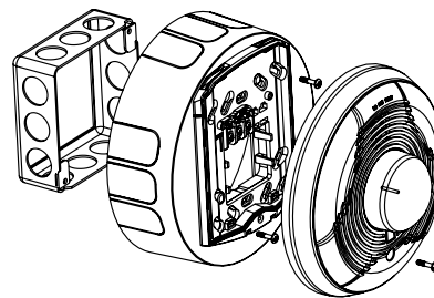
FIGURE 7. CEILING MOUNT PRODUCT WITH BACK BOX SKIRT:
